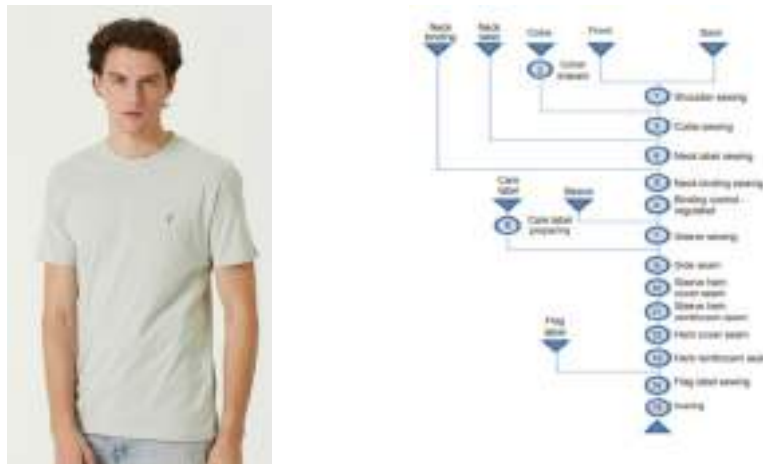
Figure 2. A Sample T-Shirt And Its Production Line
